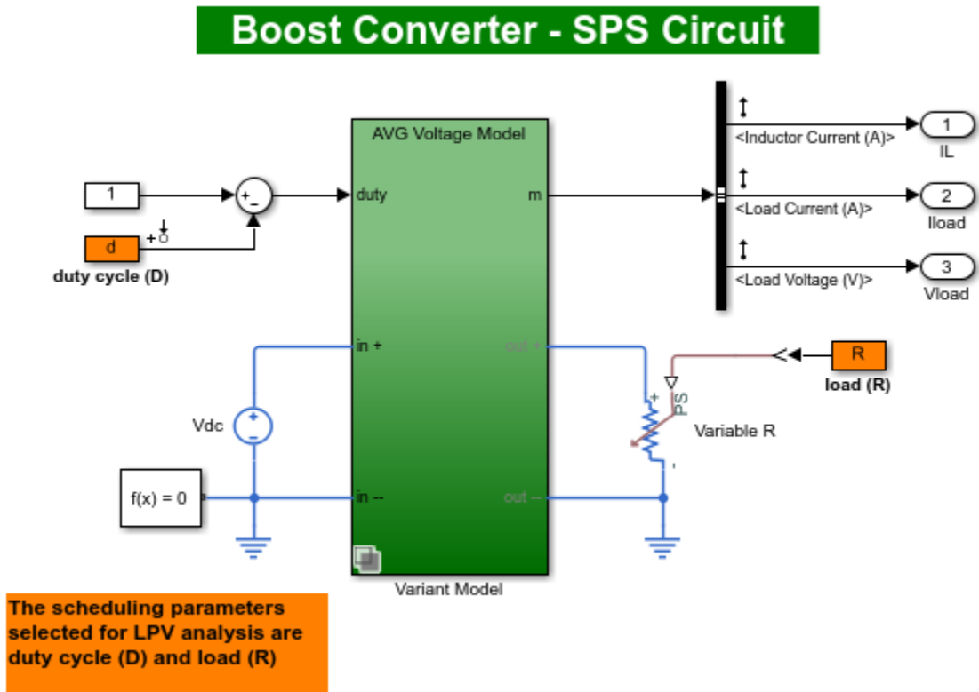
Figure 2: Simscape Electrical Power Systems based Boost Converter model
